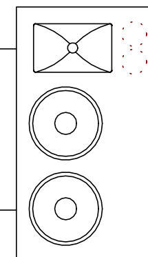
UB4770 with Network 2404H VHF Network Optional
