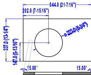
Compression Driver Support
