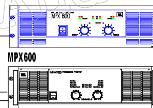
MPA1100 w/ IM-10 Xover card installed
